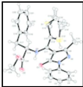
Fig. 1. The molecular structure of the title compound with the atom numbering scheme. Displacement ellipsoids are drawn at the 30% probability level. H atoms are presented as a small spheres of arbitrary radii.
